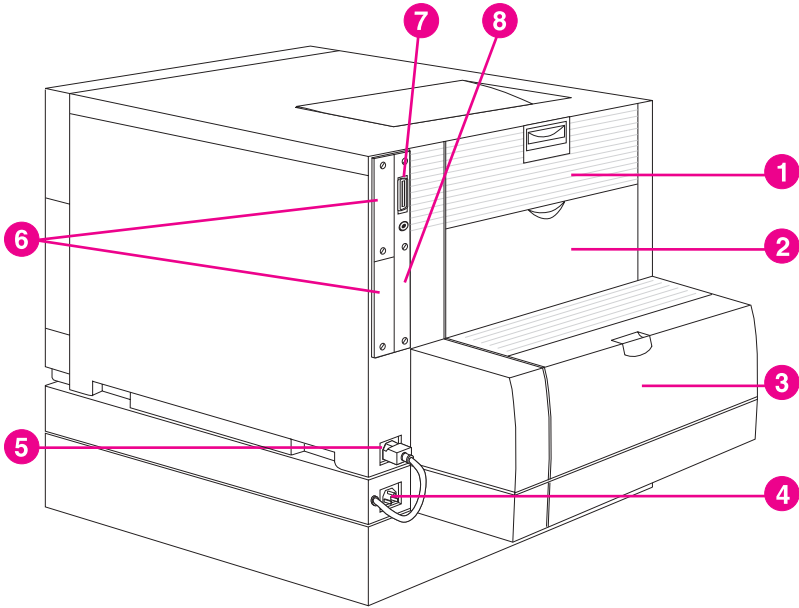
Figure 1-2 Rear View (shown with 500-sheet paper feeder and duplex printing accessory)
