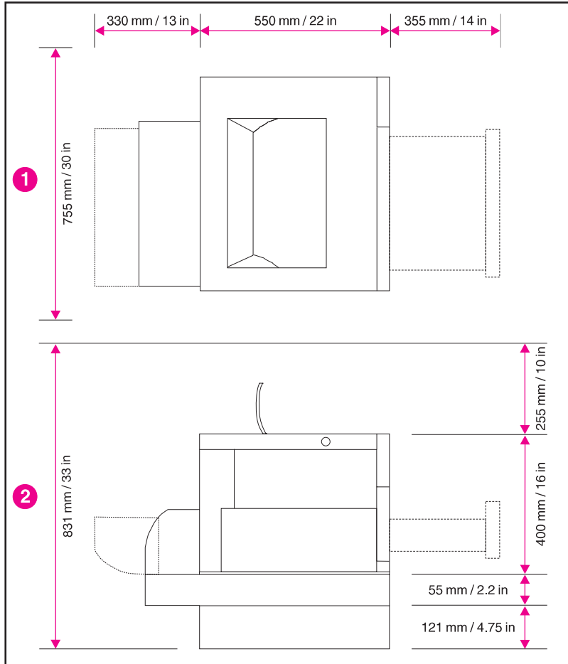
Figure 7-1 Consumable Replacement Clearance Diagram
